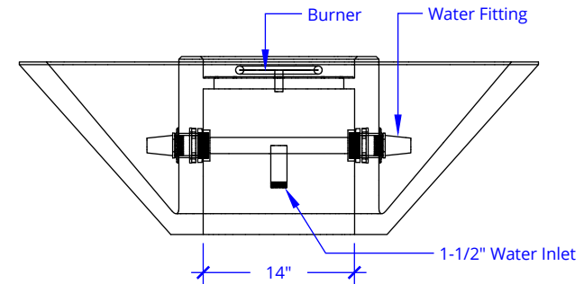
RIGHT VIEW
