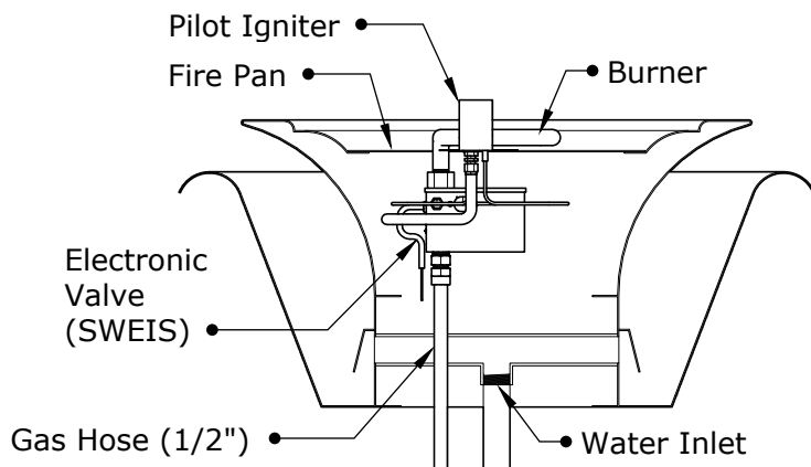
SECTION VIEW
