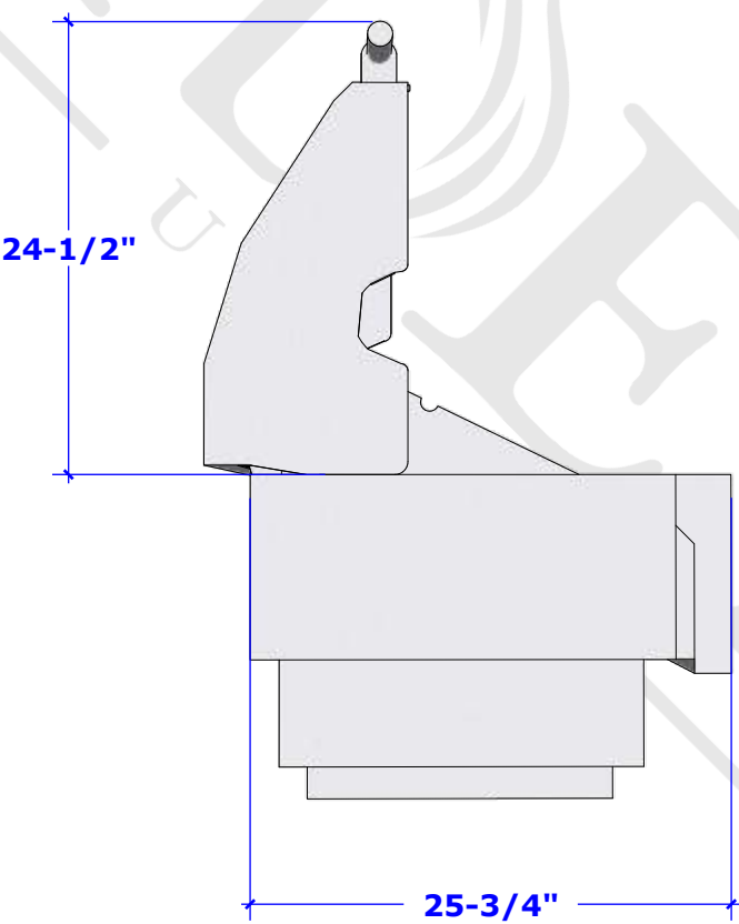
Cut Out Dimension Right Side
