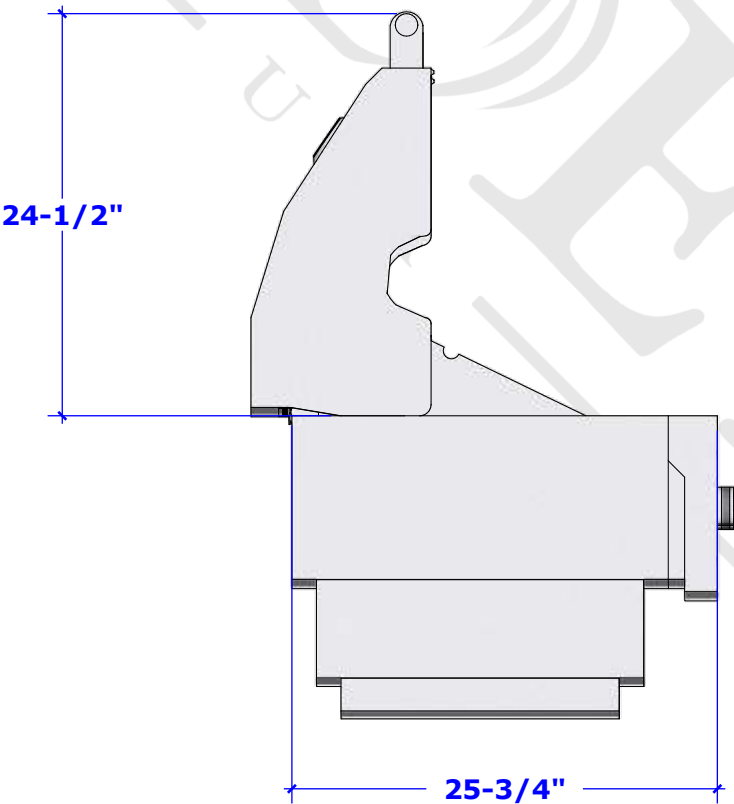
Right Side Overall Dimensions
